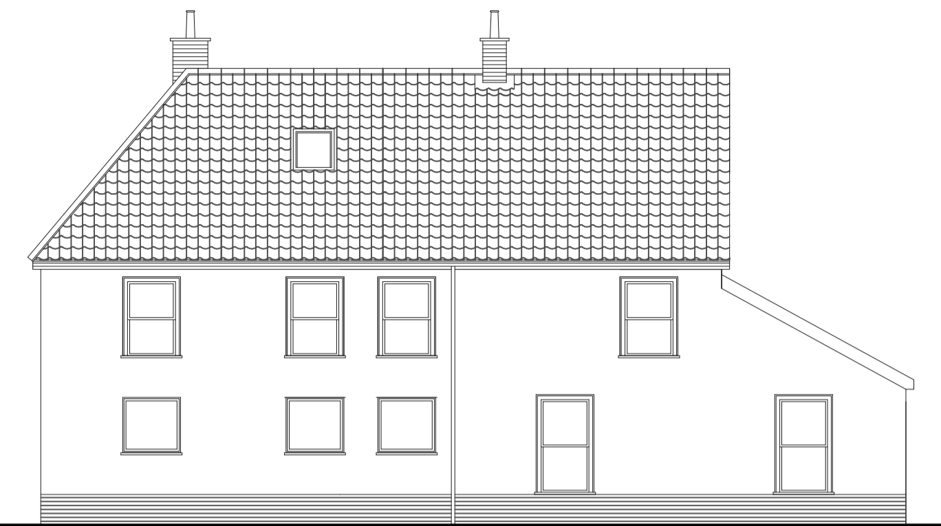
EXISTING NORTH WEST ELEVATION
